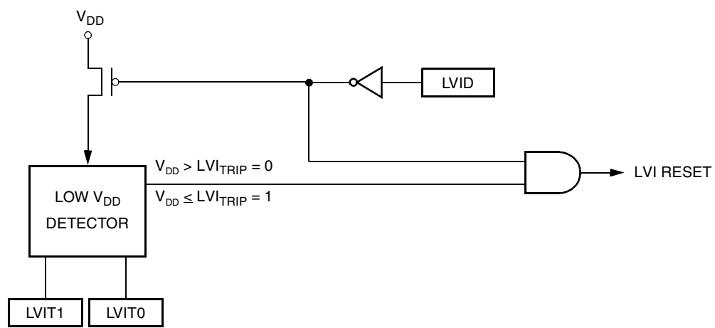
Figure 16-1. LVI Module Block Diagram
